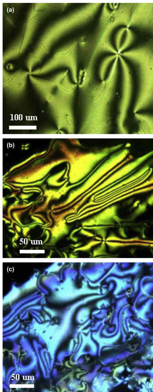
Figure 1. Polarized light microscopy images of monomers. (a) Monomer 7 : schlieren texture of nematic phase at 165 °C. (b) Monomer 8 : schlieren texture of nematic phase at 136 °C. (c) Monomer 9 : schlieren texture of nematic phase at 140 °C.
