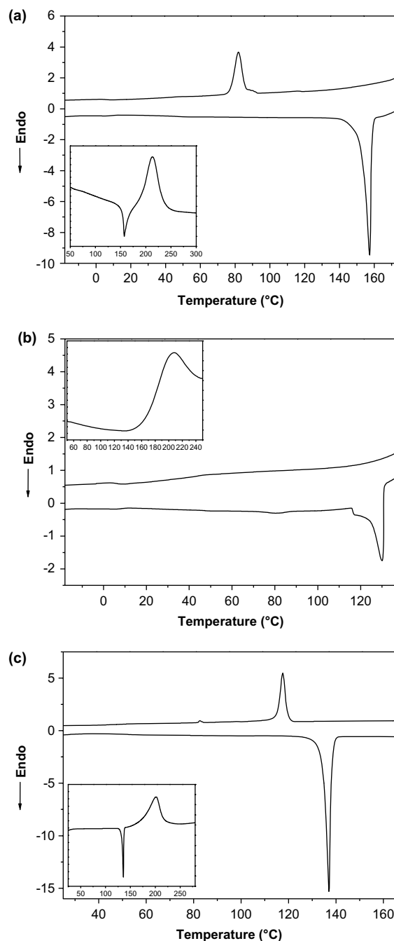
Figure 2. DSC traces for monomers on second heating and subsequent cooling. (a) Monomer 7 : from -20 to 170 °C (scan rate 10 °C min -1 ). Inset: DSC traces on third heating from 50 to 300 °C. (b) Monomer 8 : from -20 to 138 °C (scan rate 10 °C min -1 ). Inset: DSC traces on third heating from 50 to 250 °C. (c) Monomer 9 : from 20 to 165 °C (scan rate 10 °C min -1 ). Inset: DSC traces on third heating from 25 to 300 °C.
