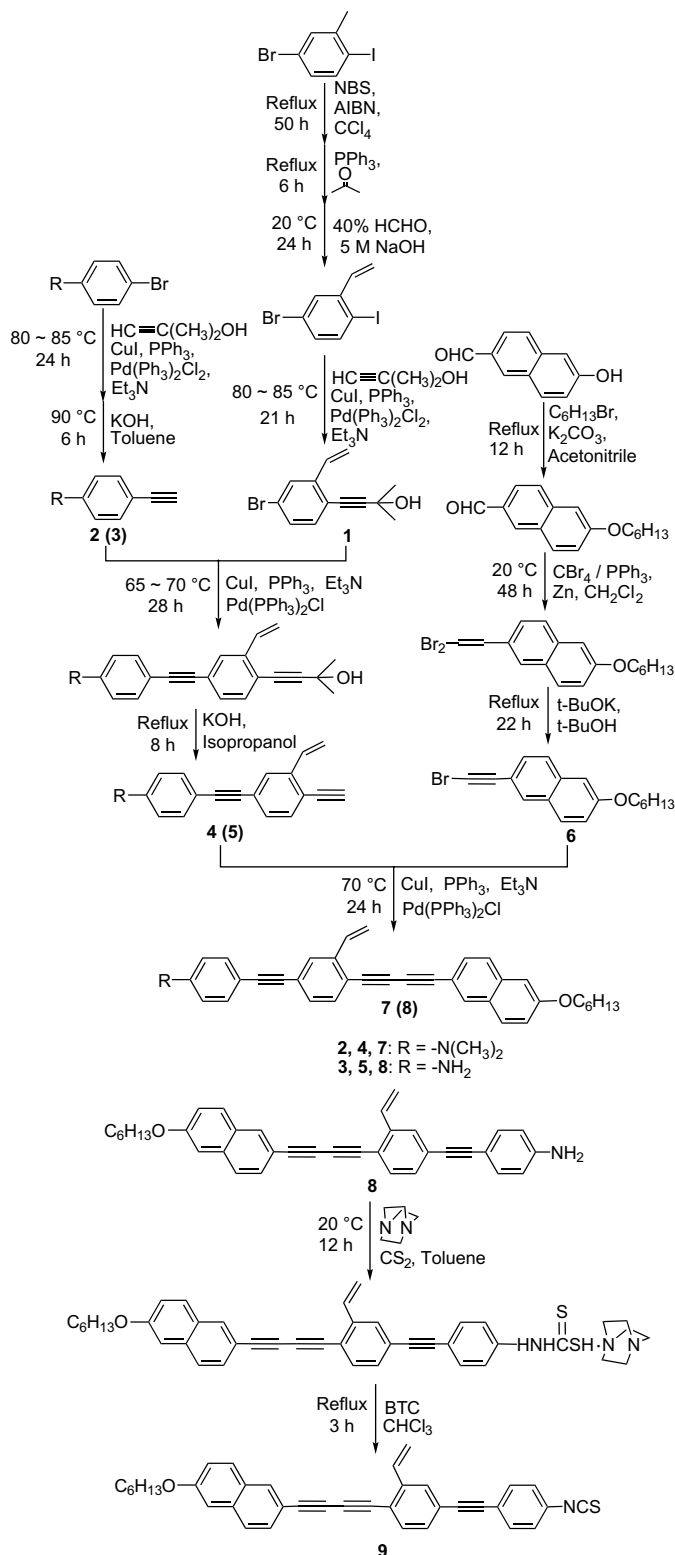
Scheme 2. Synthesis of styrene liquid crystalline monomers.
